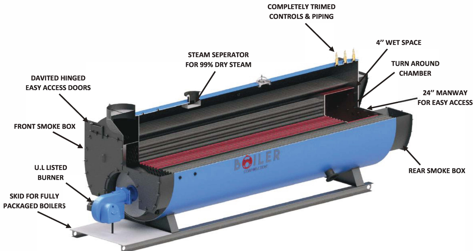
BOILER SECTIONAL VIEW
